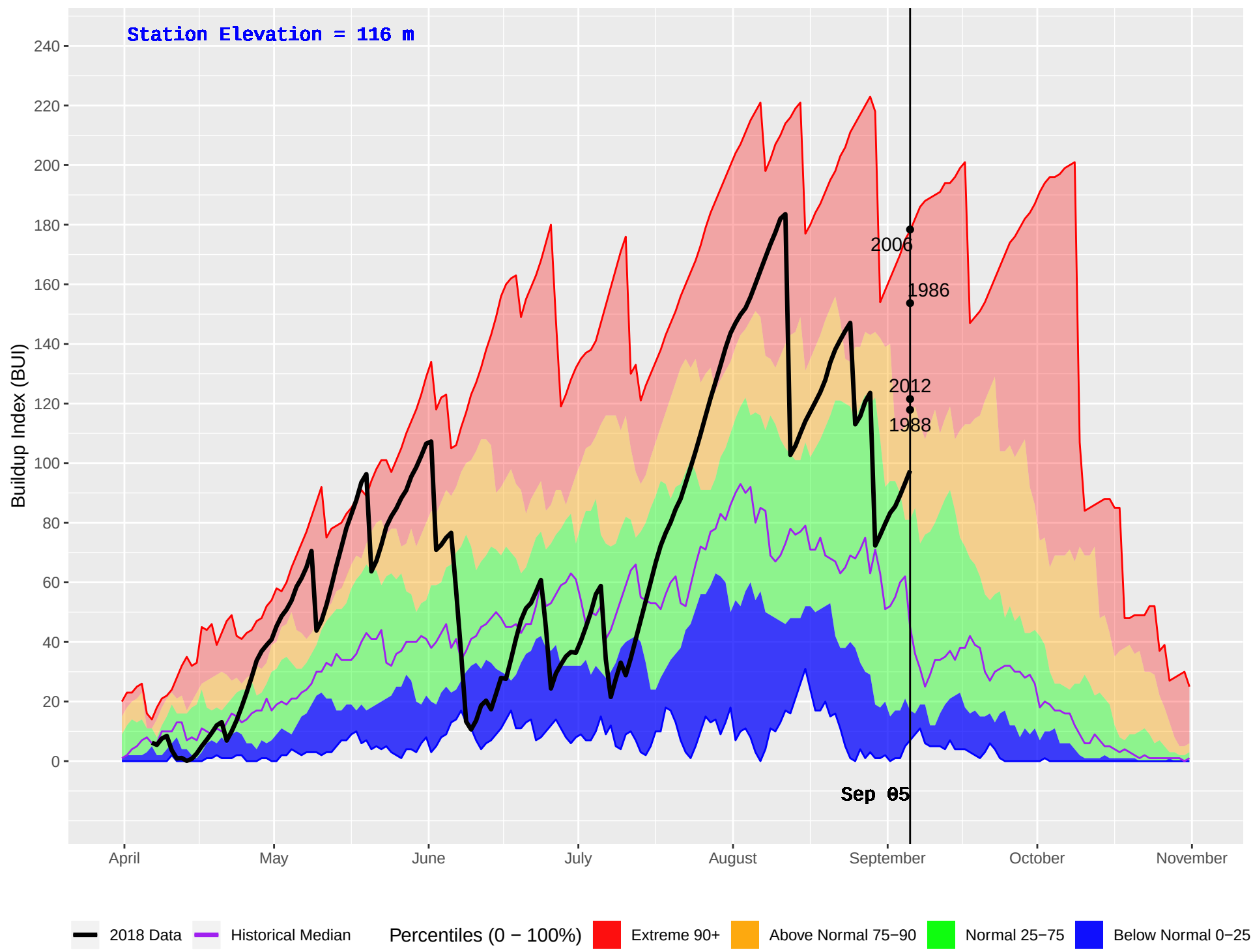
SCAR CREEK (82) : Historical (1982–2016) and Current (2018) Daily Buildup Index (BUI)
